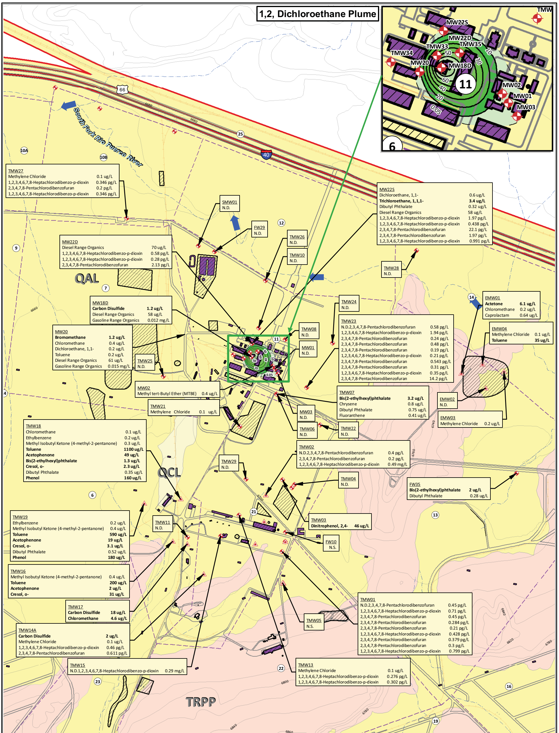
FIGURE 5-3 Northern Area VOCs, SVOCs and DRO/GRO Concentrations
