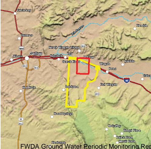
Ft. Wingate Army Depot Property Boundary Indicated in Yellow Northern Area Alluvial Ground Water Map Area in Red
