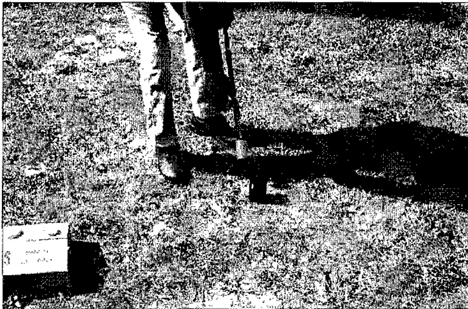
Figure 4. Coring tool (4.5-cm) used to collect discrete samples at Fort Hood, Texas.
