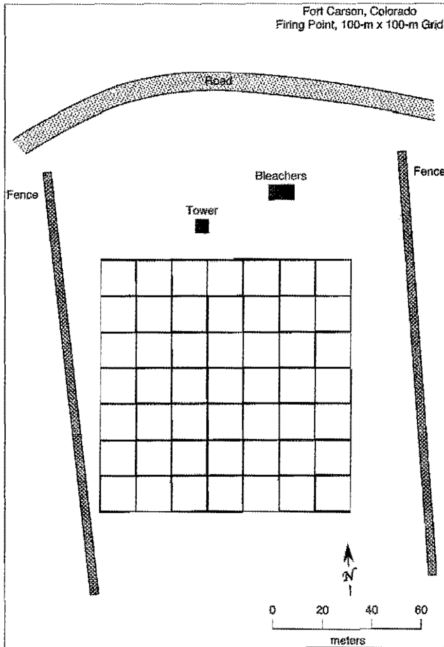
Figure 13. Diagram of 100-m x 100-m sampling grid established at a fenced-in mortar firing point at Fort Carson, Colorado.
